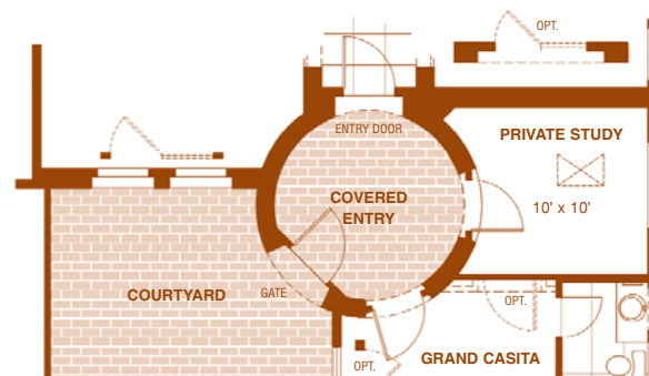
PRIVATE STUDY OPTION OFF COVERED ENTRY
